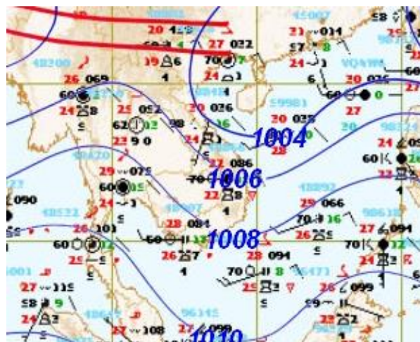
Figure 2: Weather map for 23 rd August 2015
