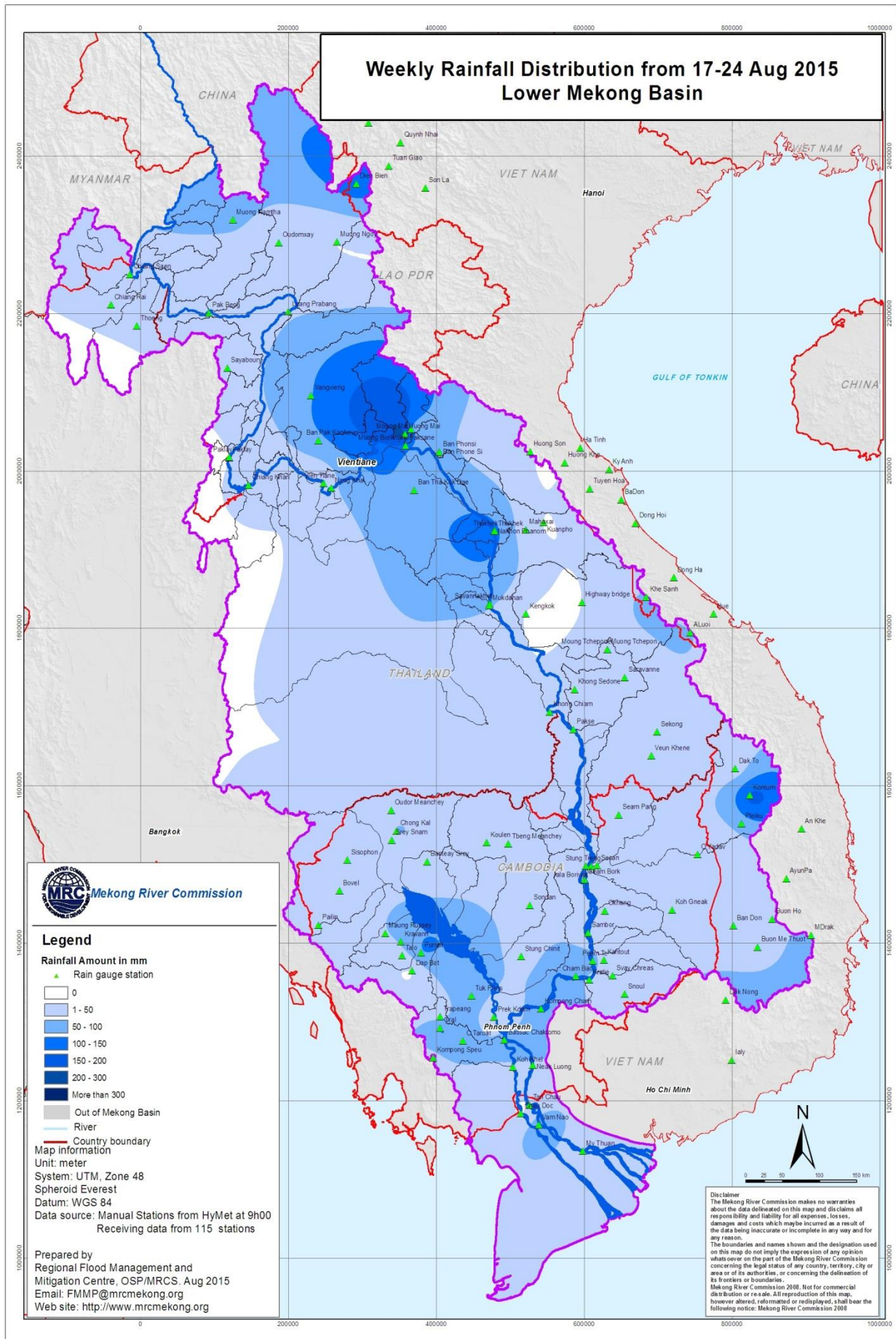
Figure 3: Weekly Rainfall Distribution over the LMB from 17 th – 24 th August 2015
