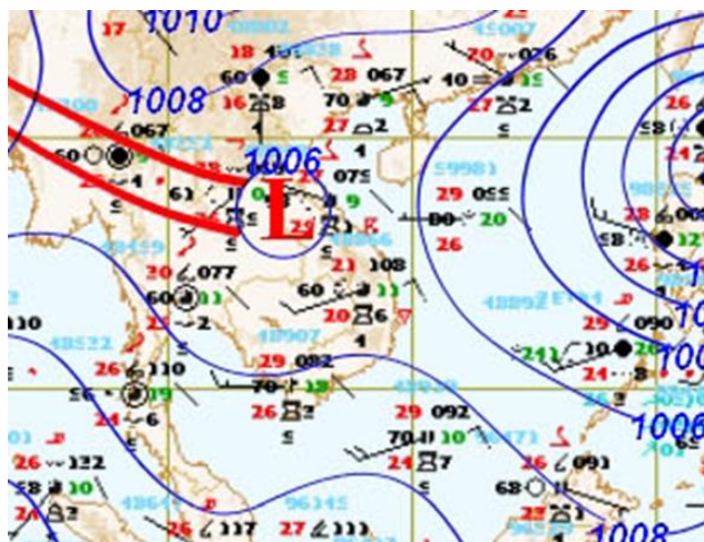
Figure 1: Weather map for 20 th August 2015
